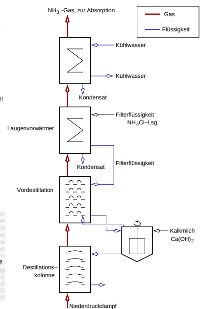
NH 3 -Stripping H
