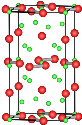
\text{Ca}_5\text{Si}_3
