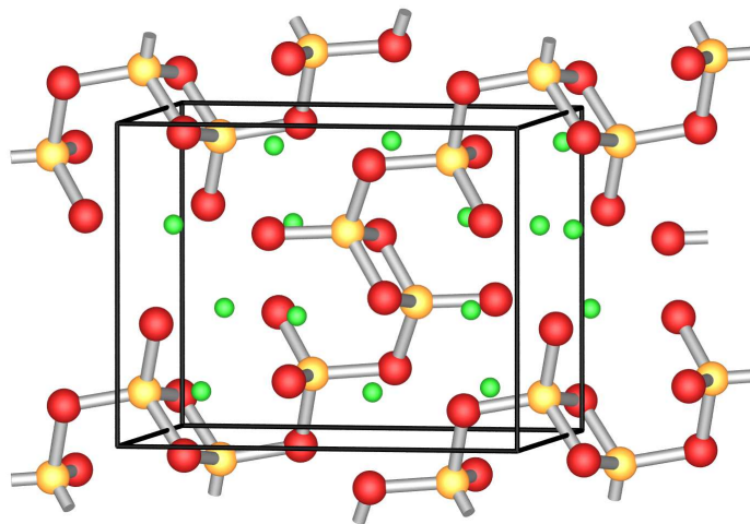
\text{Na}_7\text{In}_3\text{Se}_8
