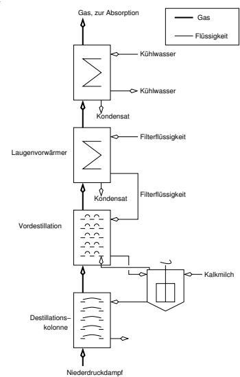
NH 3 -Stripping
