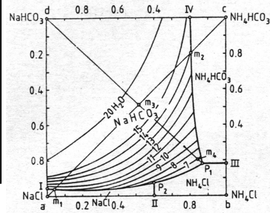
Diagramm \text{Na}_2\text{CO}_3 - \text{NH}_4\text{Cl} - \text{NaHCO}_3 - \text{NH}_4\text{HCO}_3
