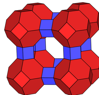
Zeolith-A
