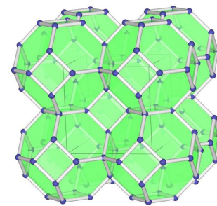
Sodalith
